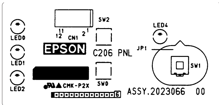
Figure A-13. C206PNL Component Layout
