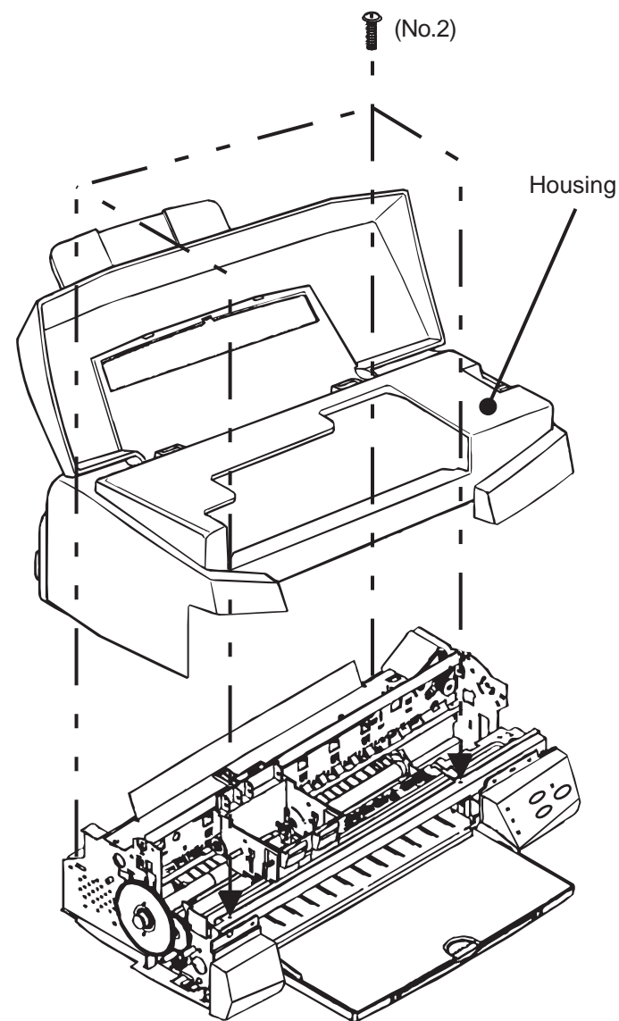
Figure 4-2. Removing the Housing
