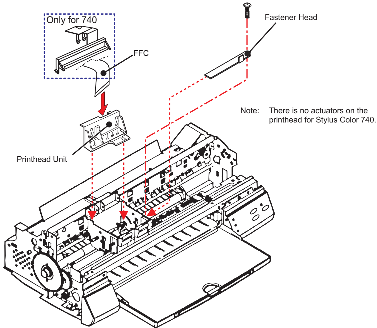
Figure 4-6. Removing the Print Head
