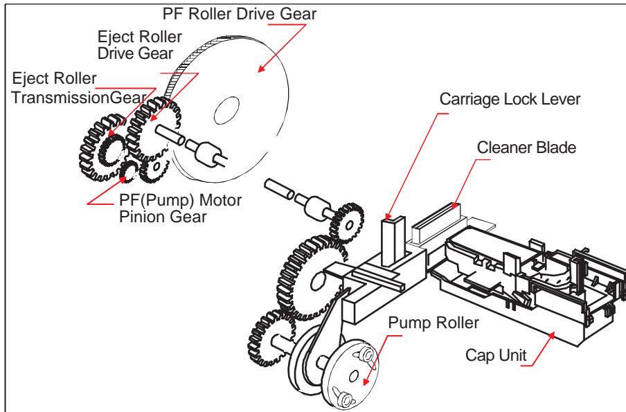
Figure 2-10. Ink System Mechanism
